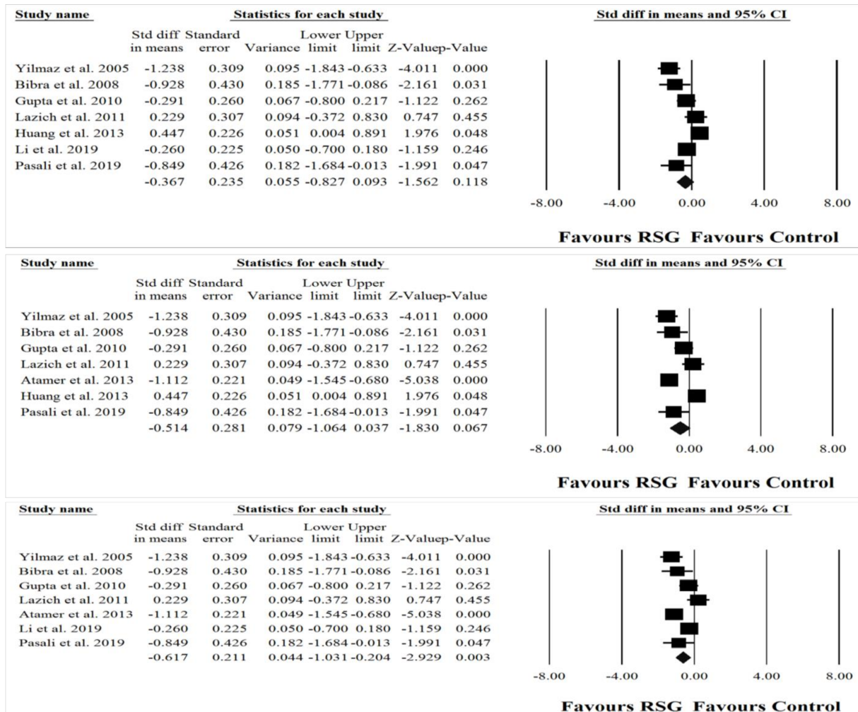
Supplementary figure 1. Leave-one-out sensitivity analyses of the effect of rosiglitazone treatment on circulating MDA level with remove the studies with low quality and the study with a large sample size in subjects with T2D. Meta-analysis was performed using a random-effects.
